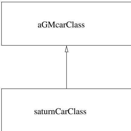
Generalization Relationship
