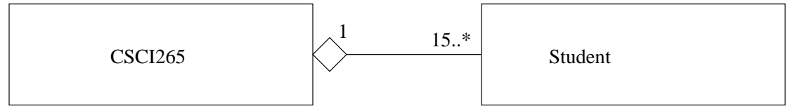
Aggregation Relationship
