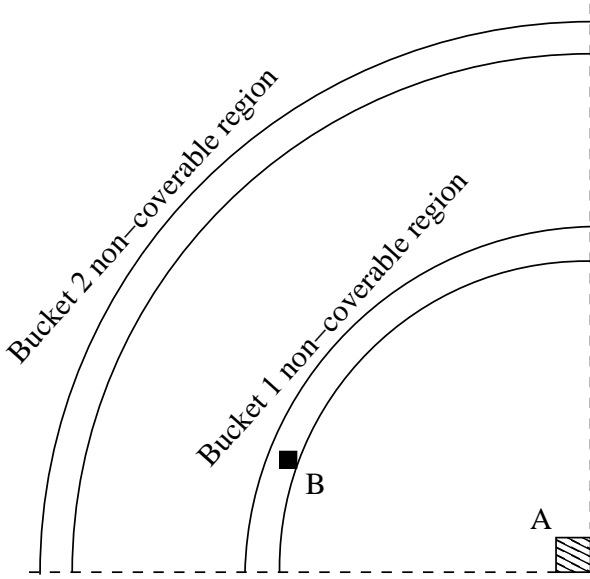
Fig. 14 A cell with a large number of data points in 2D space and its first two non-coverable regions (one the lowest level of the ). The cell is denoted as cell A and non-coverable regions are represented by annuli (rings). Only one quarter of the regions are plotted.
