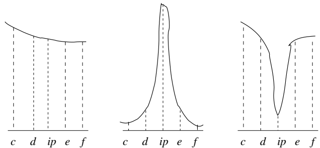
Fig. 13 Three cases of distribution of distances around the edge of buckets i and i + 1 , with the solid curves representing portions of the density function of the distances; [c, d] and [e, f] are examples of distance ranges of resolvable subcells. Those of the non-resolvable subcells are not shown. Line segments are not drawn on scale. For example, ip does not have to be the middle point of [c, f] in practice.
