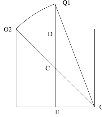
Fig. 5 A magnification of region B (i.e., QQ_1Q_2Q_3 formed by four arcs in Fig. 4). Here we only show arc Q_1O_2 , which is a half of arc Q_1Q_2 .
